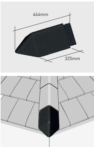
Q93*K | Hoekkeper beginvorst
