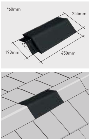
Q90*K | Atica ridge 120° klinker
